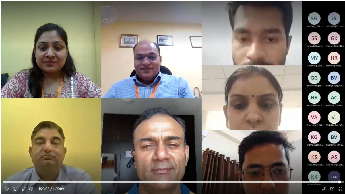
Figure 6: Query session
